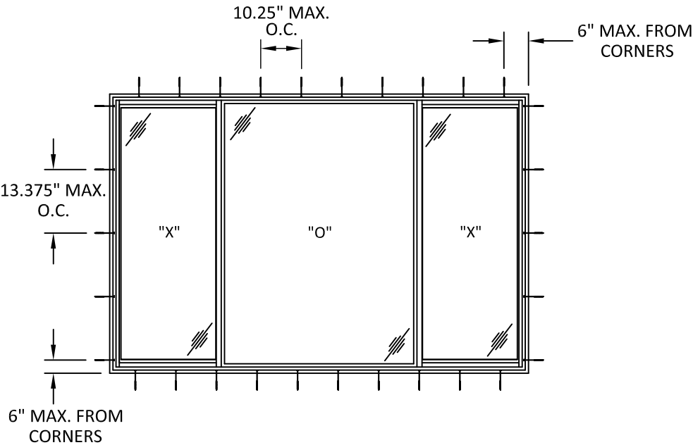
TYPICAL ANCHOR LAYOUT THROUGH FRAME AND CLIP INSTALLATION
