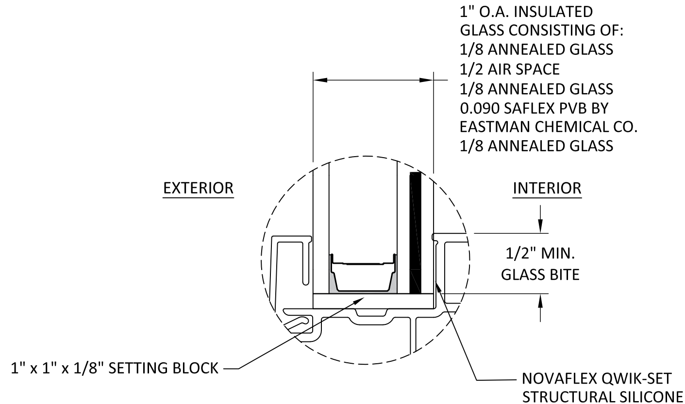
GLAZING DETAIL
