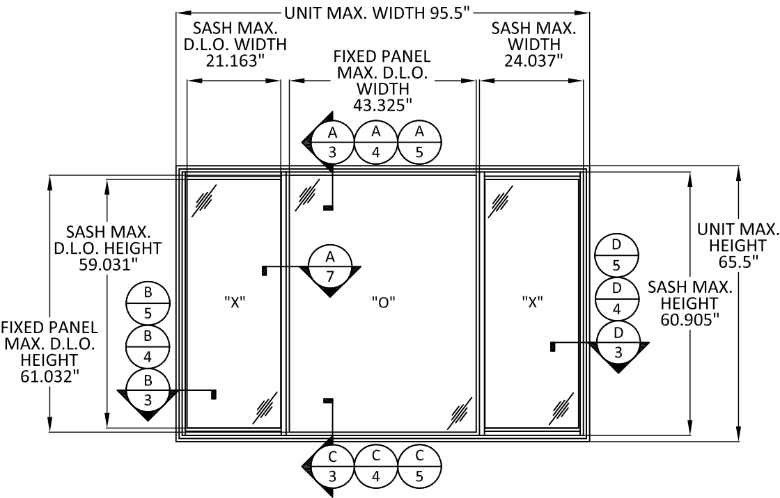
TYPICAL ELEVATION HORIZONTAL SLIDER END VENT WINDOW
