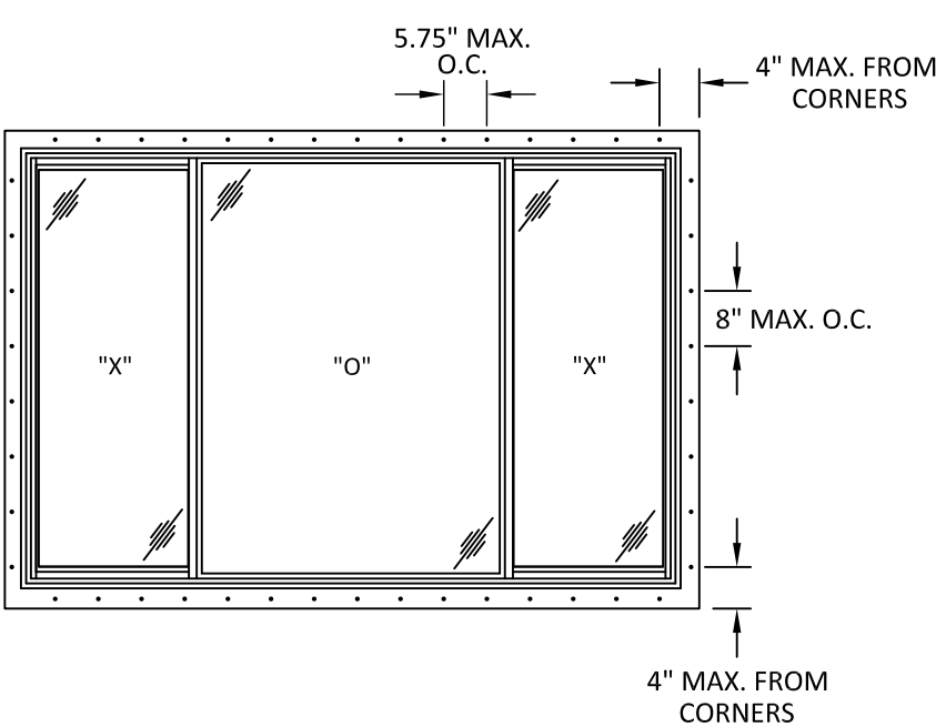
TYPICAL ANCHOR LAYOUT NAIL FIN INSTALLATION
