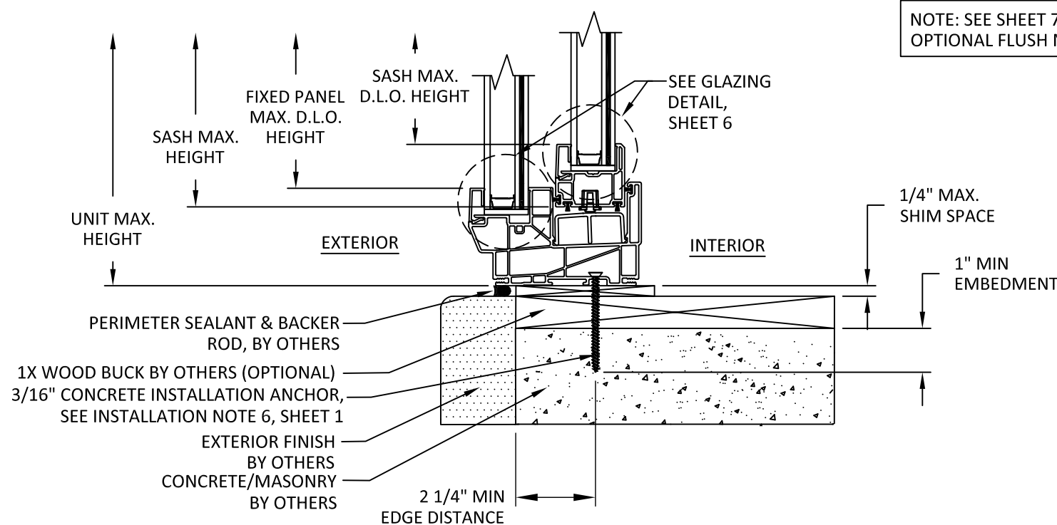
C 4 VERTICAL SECTION THROUGH FRAME INSTALLATION CONCRETE/CMU
